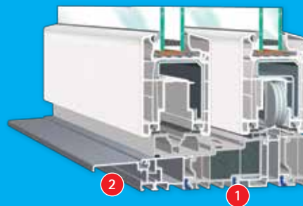
4- panel solution with 2 lift and slide sashes and 2 fixed panes
